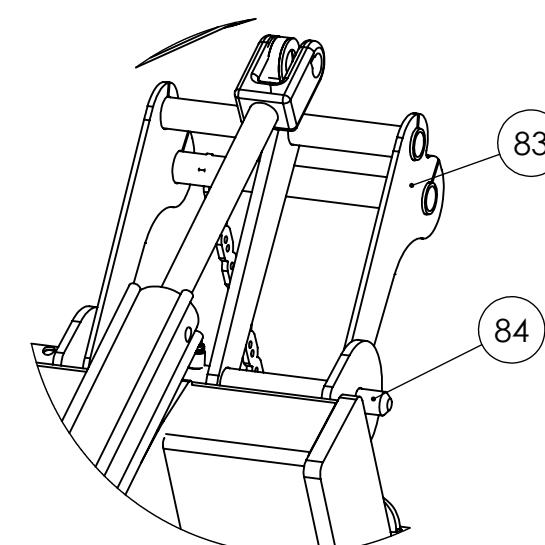
83 84 DETAIL AA 1:8 Typical Two Places
