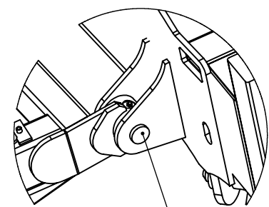
38 DETAIL N 1:12
