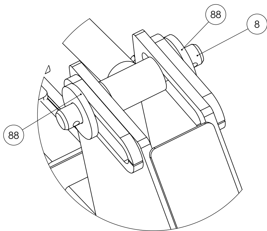
88 8 DETAIL P 1:4
