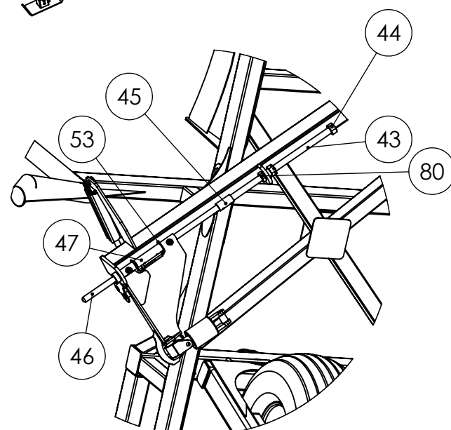
44 45 43 80 47 46 Rear Center Chain Adjustment Details
